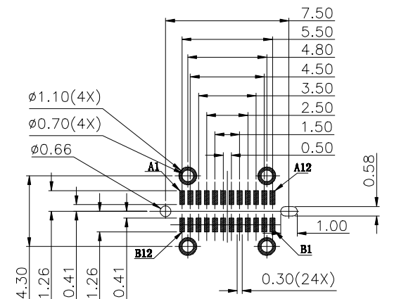
RECOMMENDED PCB LAYOUT(TOP VIEW) THICKNESS 1.5±.10MM;DEFAULT TOLERANCE:±.05
