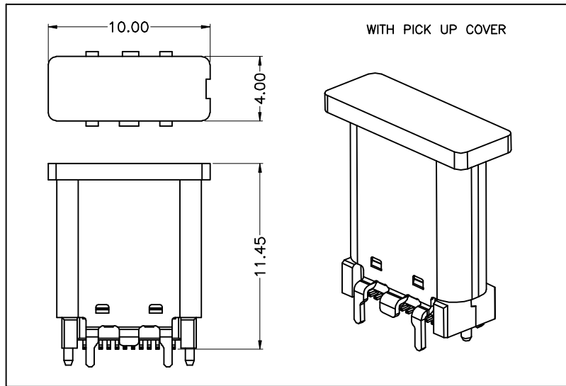
USB TYPE-C PIN ASSIGNMENTS
