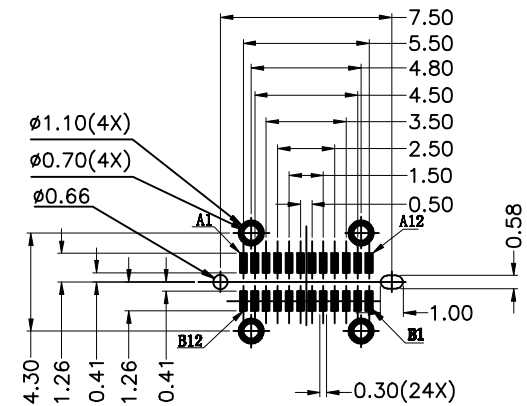
RECOMMENDED PCB LAYOUT(TOP VIEW) THICKNESS 1.5 \pm 0.10MM;DEFAULT TOLERANCE: \pm 0.05
