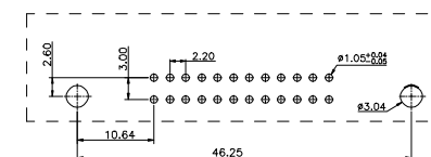
SECTION F-F
