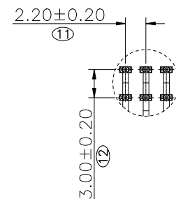
DETAIL G SCALE 2:1
